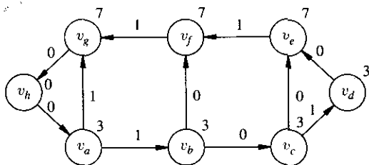
FIGURE 9.10 Retimed network.
