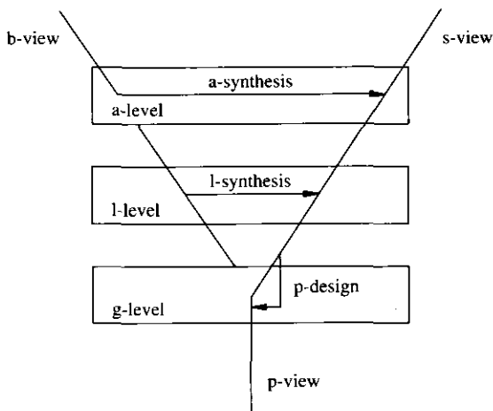
FIGURE 1.11 Levels of abstractions, views and synthesis tasks.
