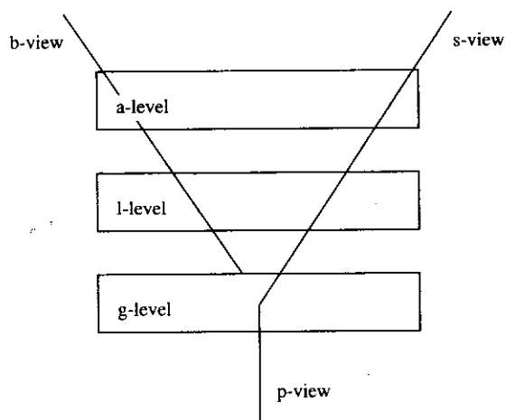
FIGURE 1.8 Three abstraction levels of a circuit representation.
