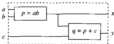
FIGURE 3.7 Example of a logic network.
