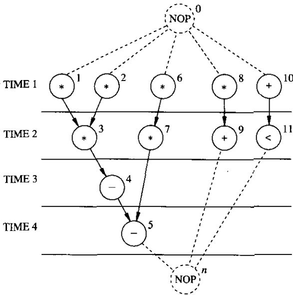
FIGURE 5.2 ASAP schedule.
