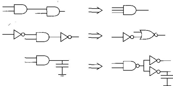
FIGURE 10.23 Two simple transformation rules.
