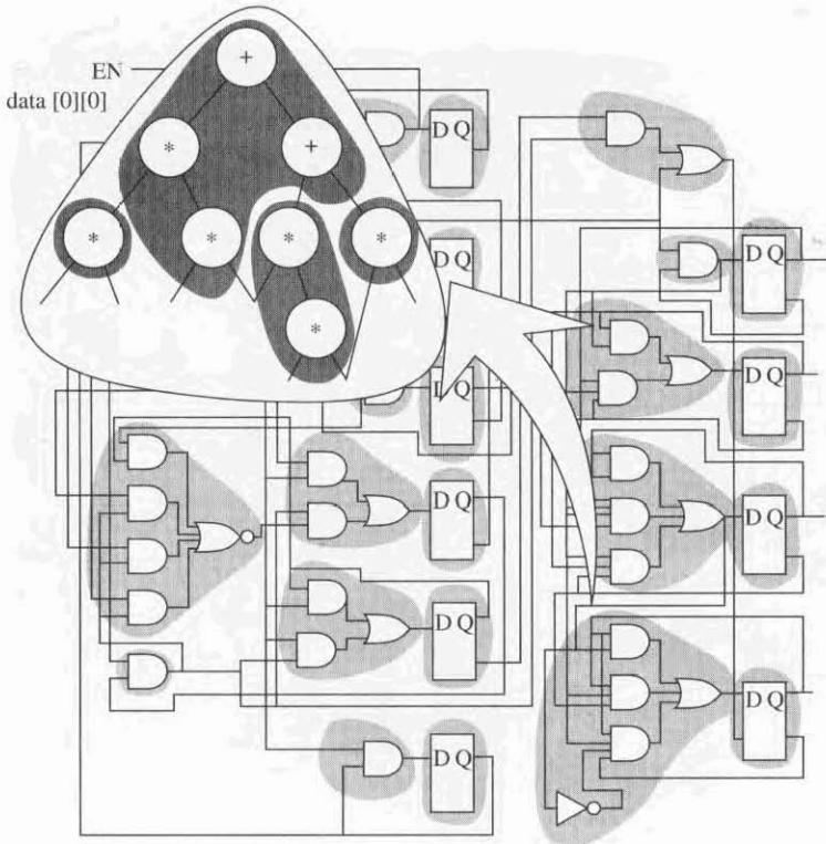
FIGURE 10.6 Covering of a subject graph.
