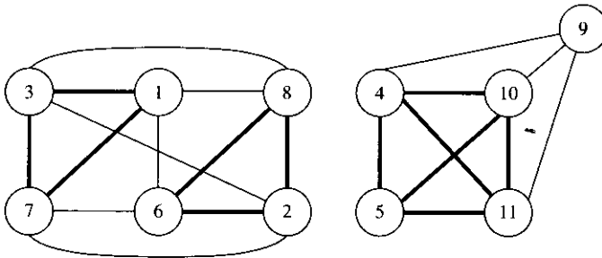
FIGURE 6.2 Compatibility graph.
