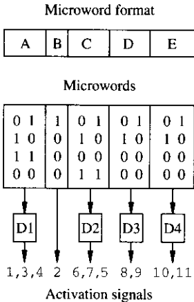
FIGURE 4.15 Example of encoded microwords using five fields.
