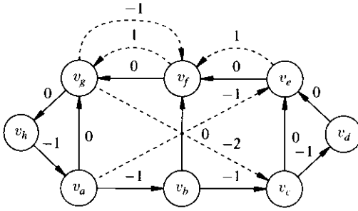
FIGURE 9.11 Constraint graph.
