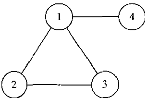
FIGURE 6.14 Compatibility graph.
